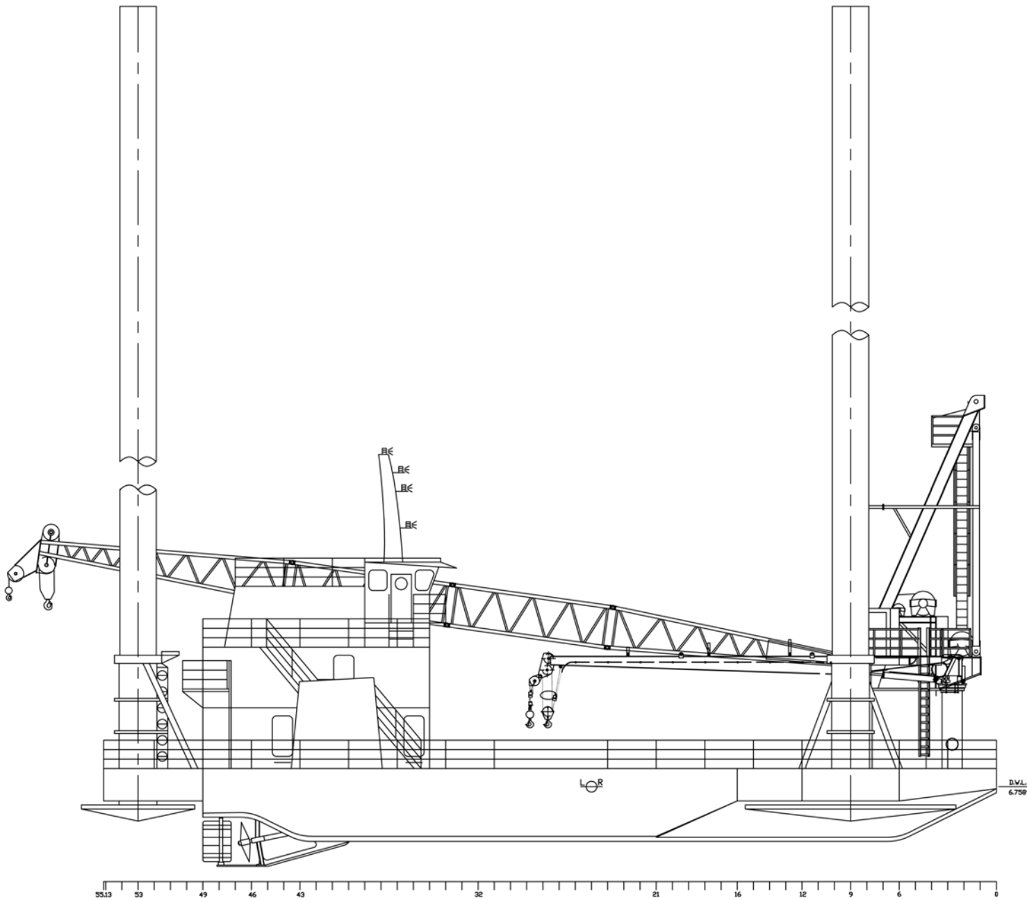
OUTBOARD PROFILE SCALE 3/16" = 1'-0"
