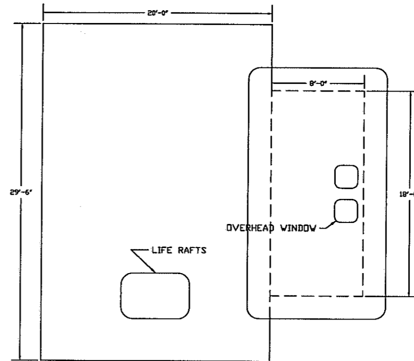
GENERAL ARRANGEMENT 04 LEVEL SCALE 1/4" = 1'-0"
